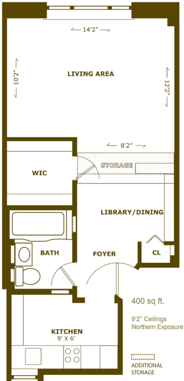
LAYOUT
